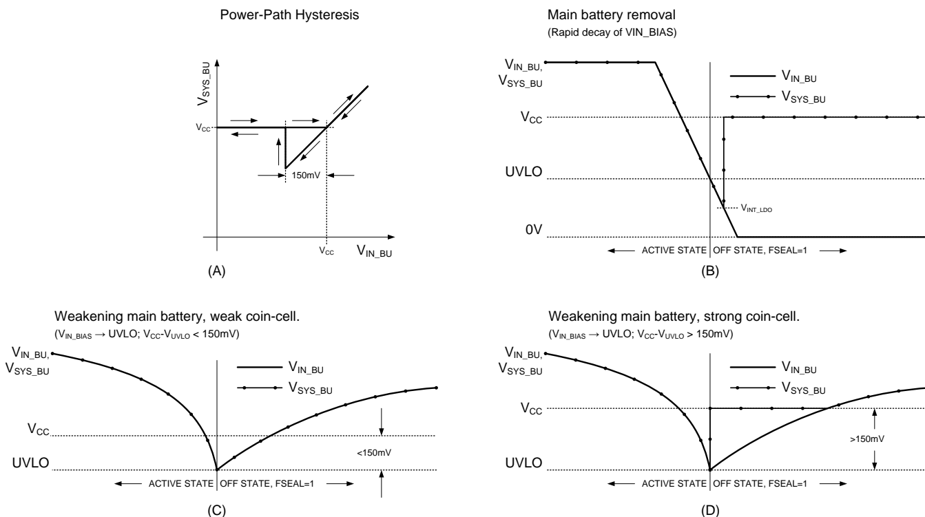
Figure 20. Switching behavior of the Battery-Backup-Supply Power-Path.
