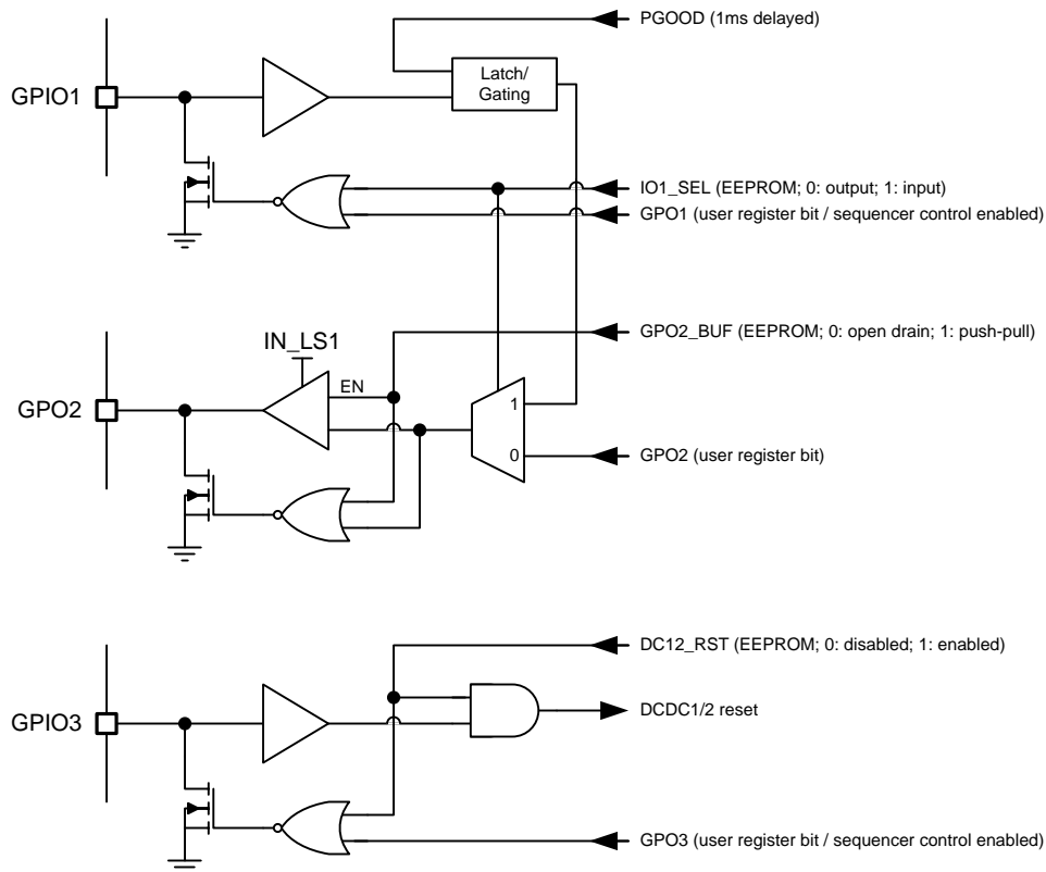
Figure 25. I/O Pin Logic
