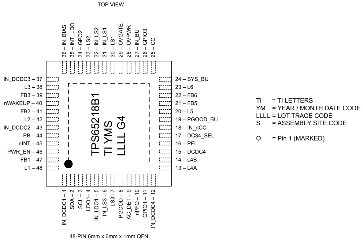
TPS65218 (TOP VIEW)
